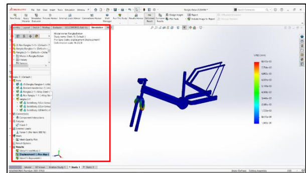
Figure 7. Strain Simulation
