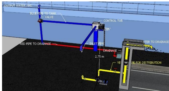
Figure 7. Piping Design
