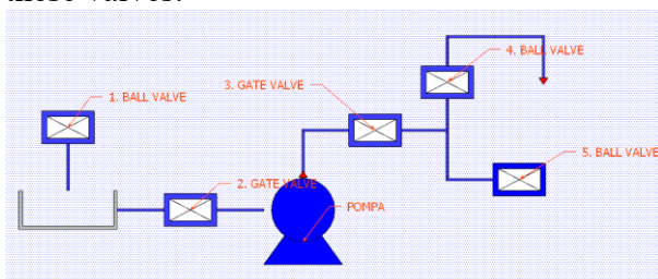
Figure 9. Blok System Valve
