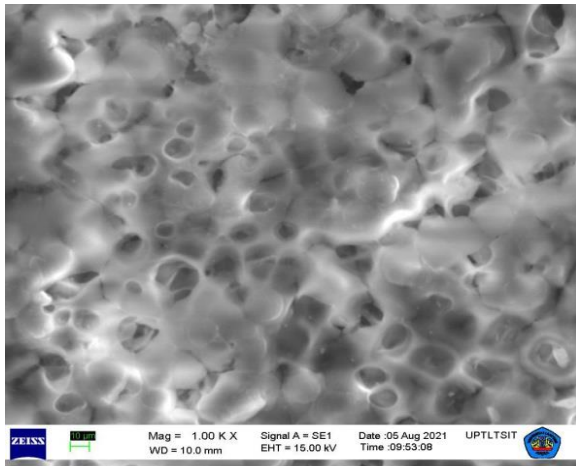
Figure 6. SEM Membran PVDF & SnO 2 17.5 wt%
