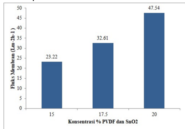
Figure 8. PVDF and SnO 2 flux graphs
